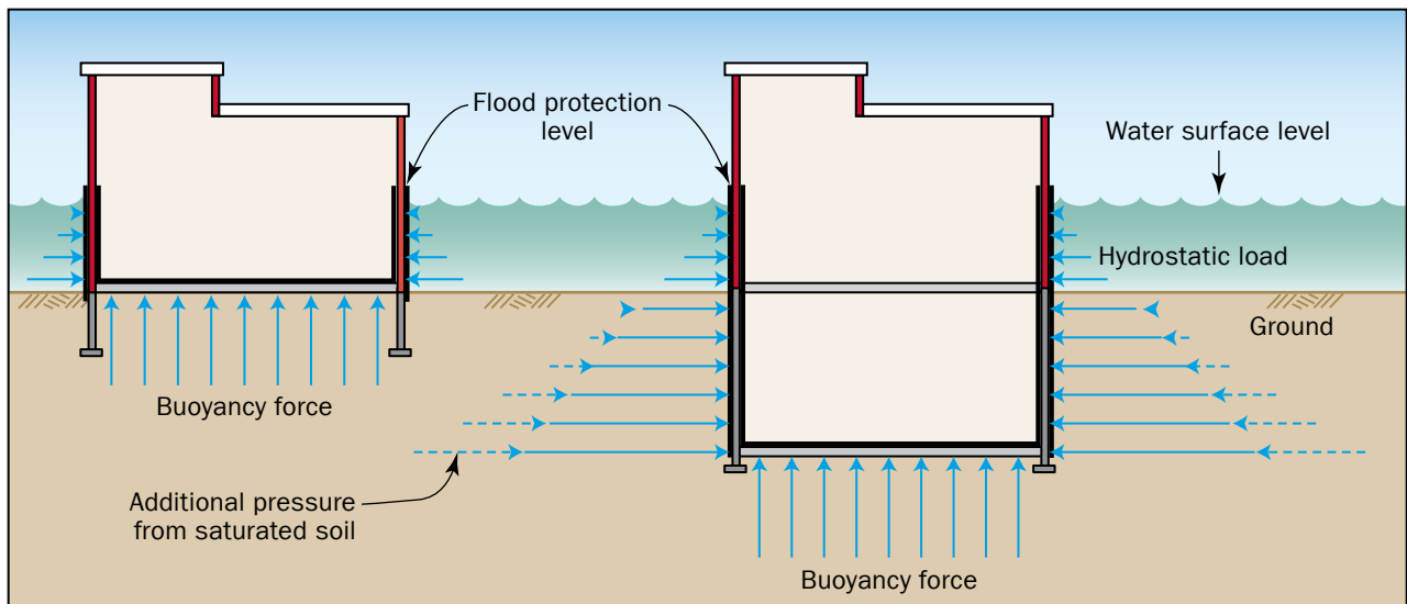
Figure 3: Hydrostatic loads
